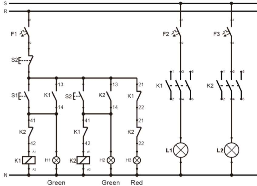
JOB ORDER 7 KENDALI MOTOR MENYALA BERGANTIAN (INTERLOCK)
